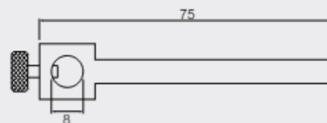
MS-SP-003 Indicator holder/Rod depth clamp
